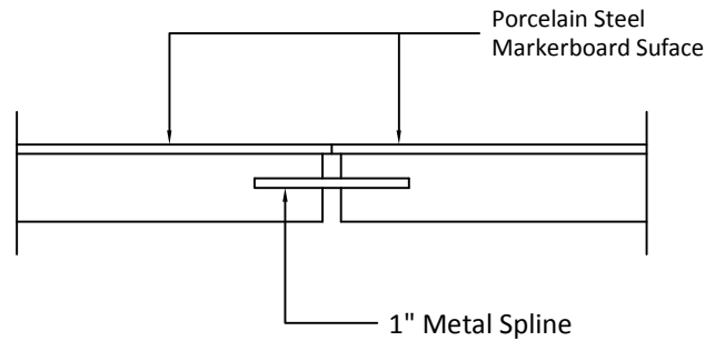
OPTIONAL SPLINED JOINTS BETWEEN MARKERBOARD PANELS
