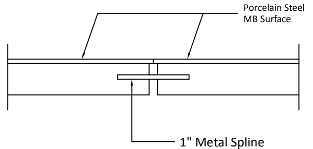
OPTIONAL SPLINED JOINTS BETWEEN MARKERBOARD PANELS
